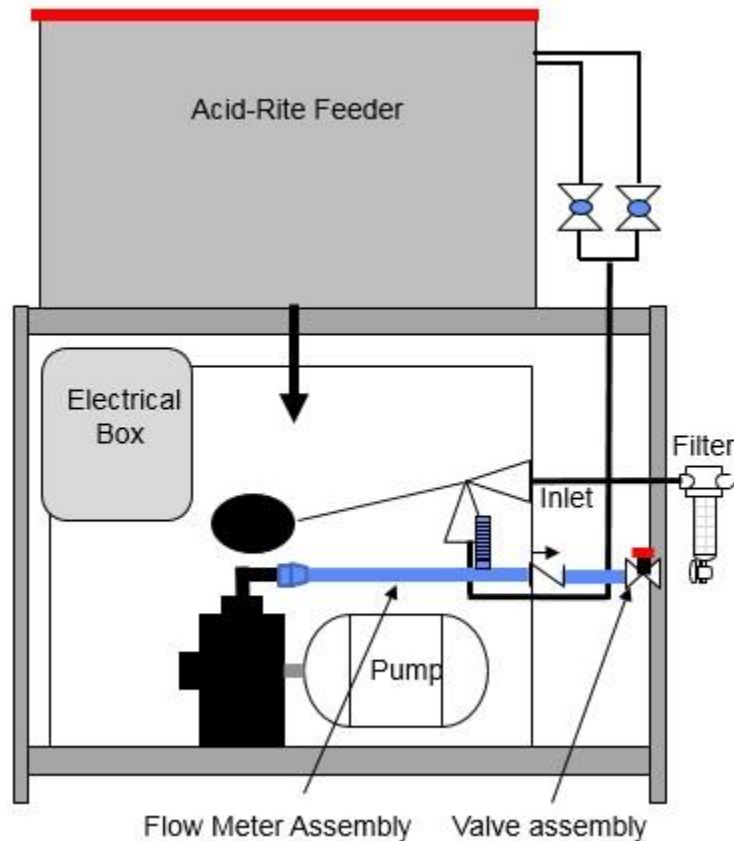
FIGURE 1 – Installation
